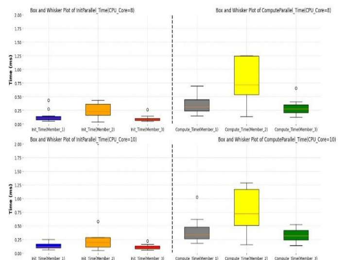
Figure 8: Comparison between initialization time ( InitParallel_Time ) and computation time ( ComputeParallel_Time ) for CPU core 8 & 10 configurations across multiple PCs.
